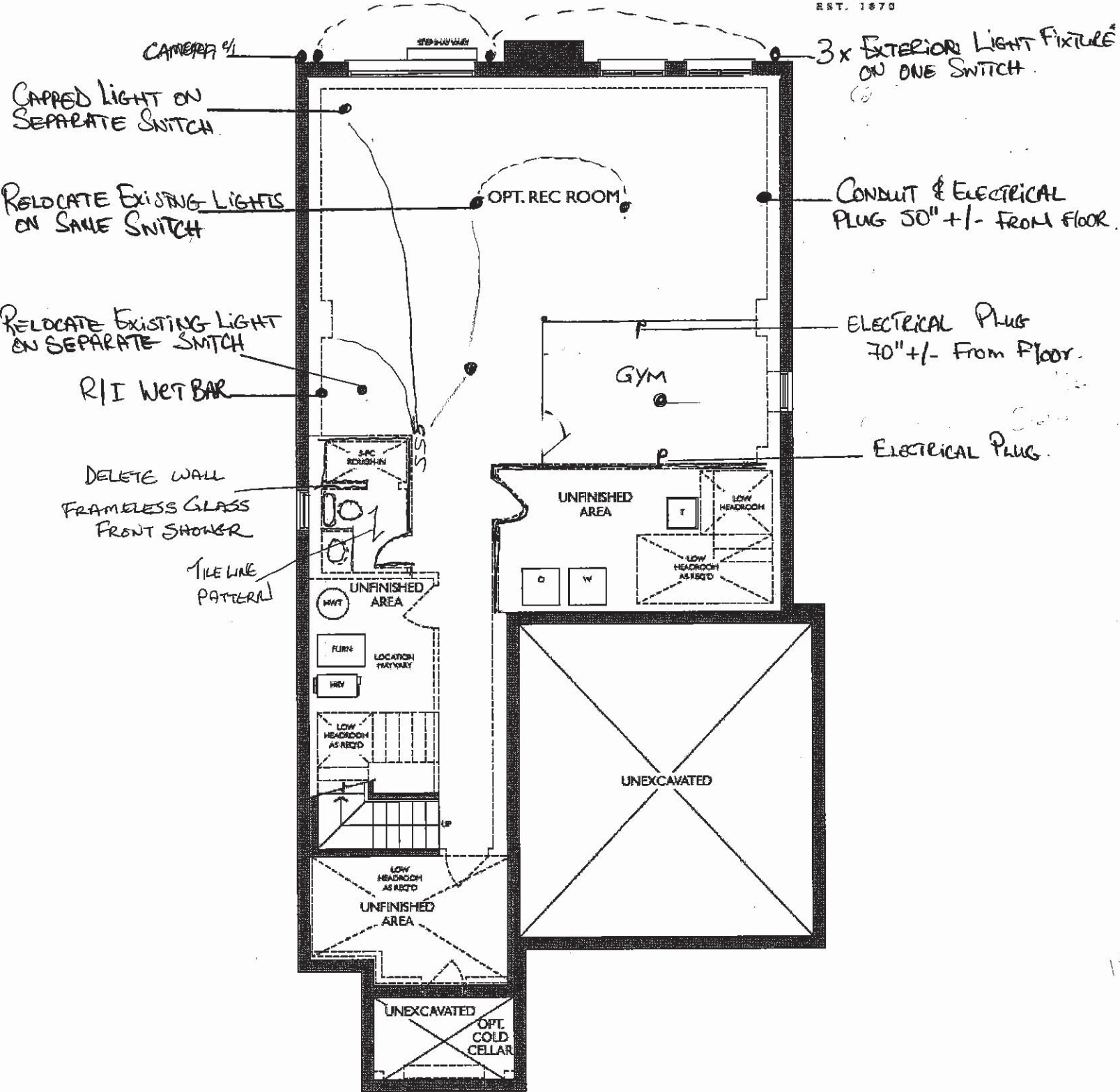
OPT. FINISHED LOWER LEVEL ELEVATION A & B
