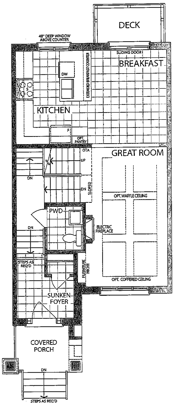
MAIN LEVEL ELEVATION A & B
