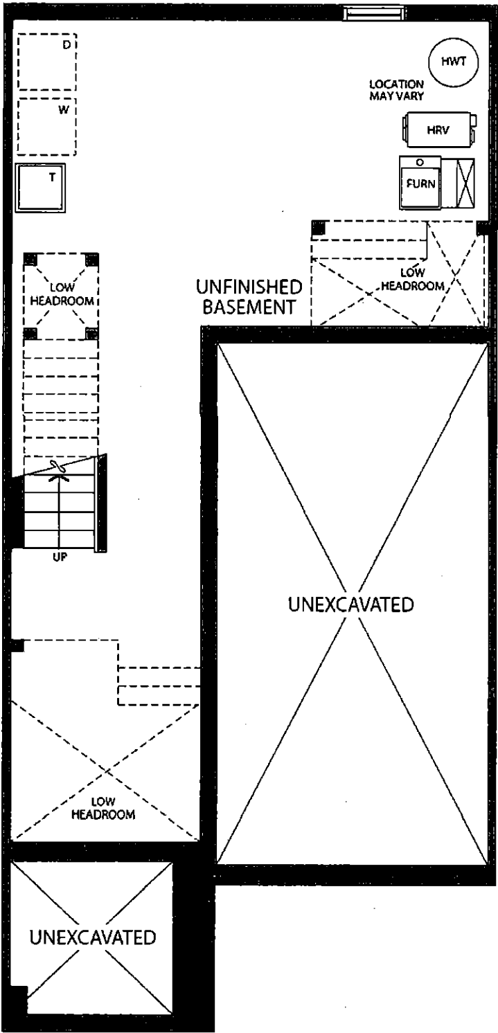
OPT. BASEMENT PLAN FOR OPT. BEDROOM 4 & BATH, EL. 'A'
