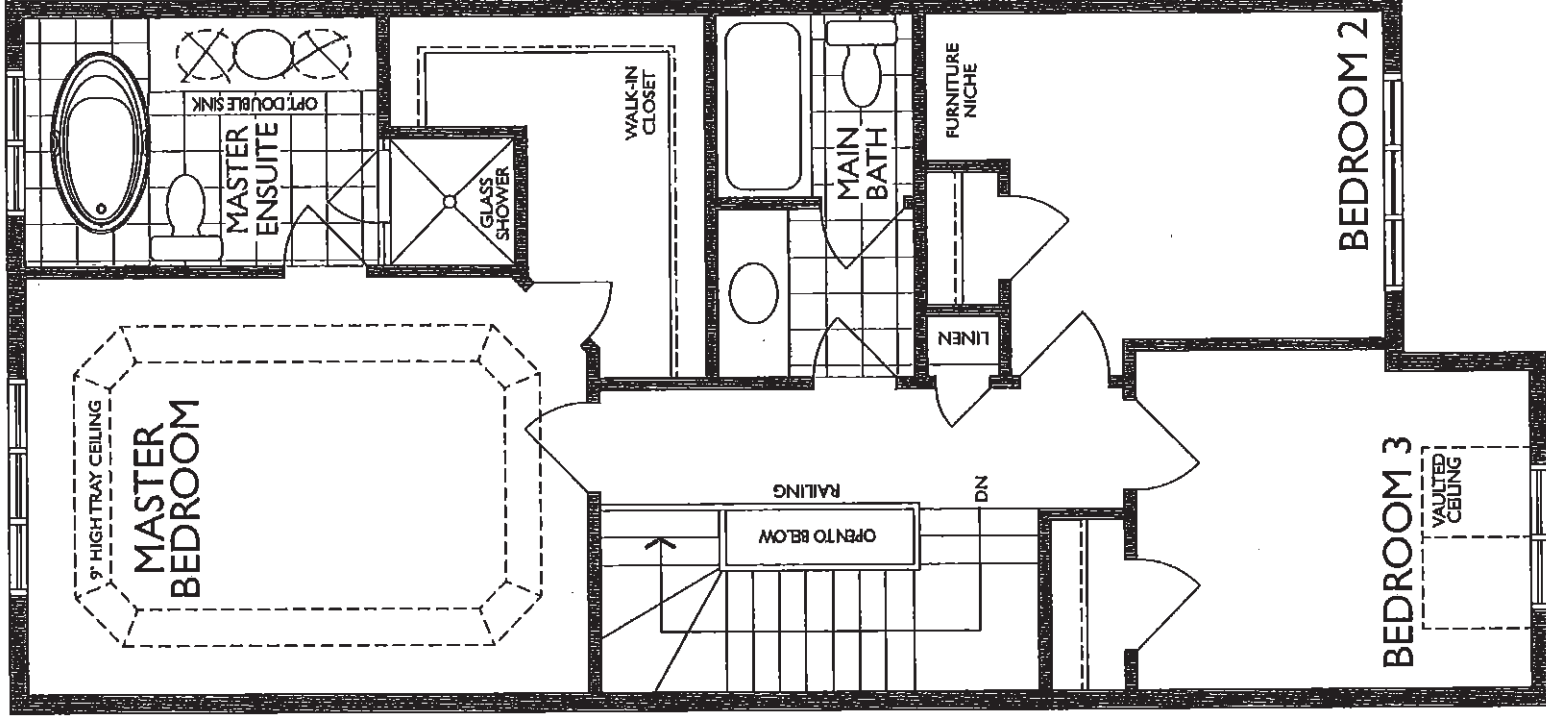
SECOND FLOOR ELEVATION A
