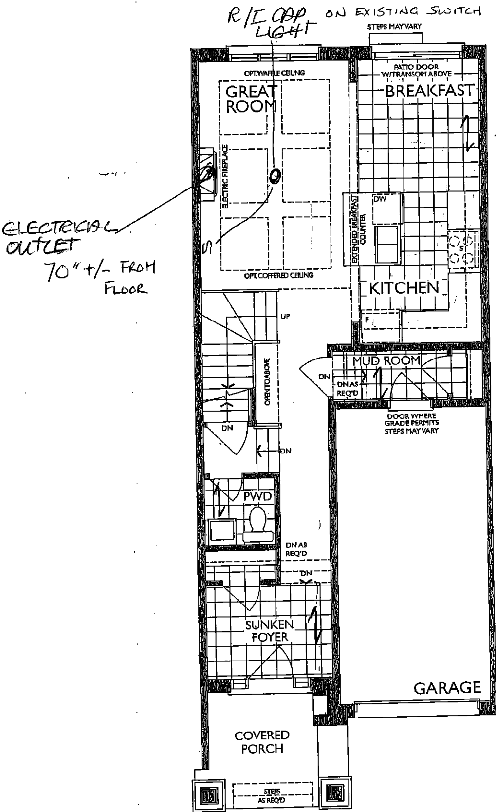
MAIN FLOOR ELEVATION B
