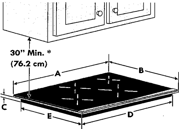
Cooktop Dimensions
