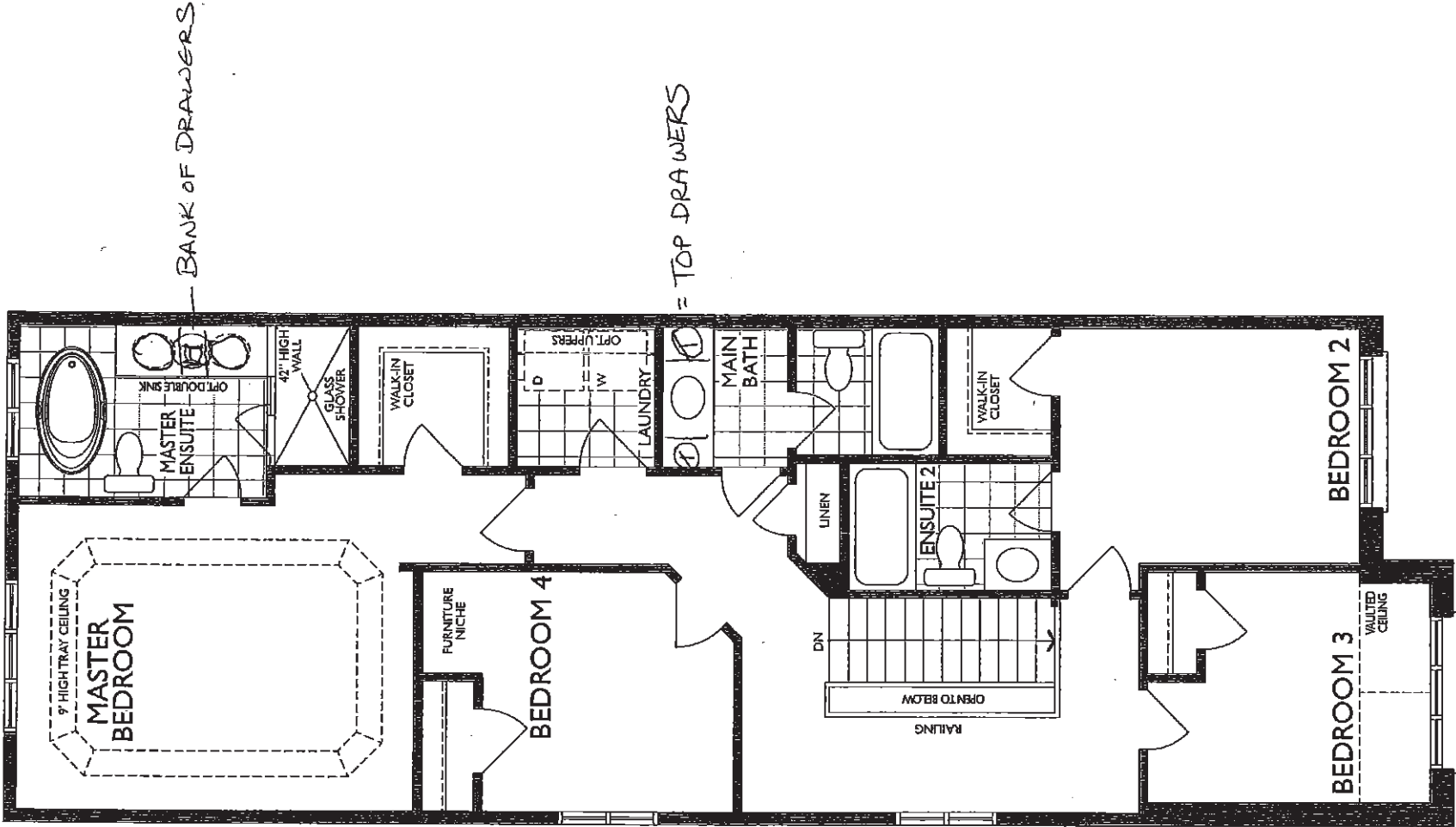
ALT. SECOND FLOOR ELEVATION B
