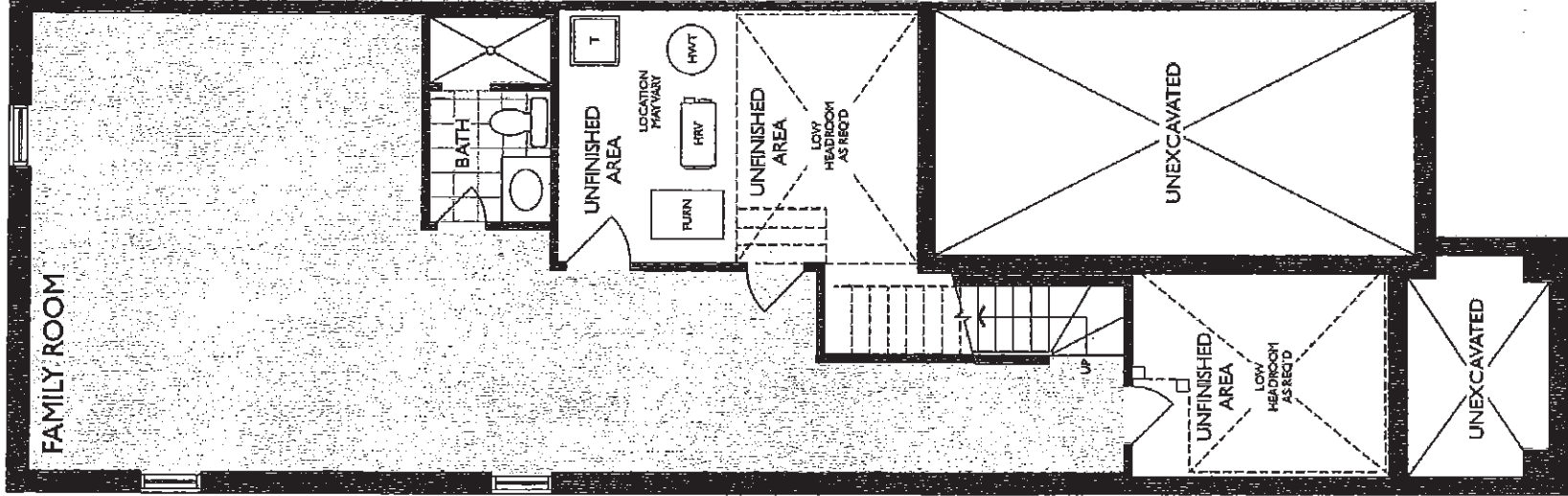
LOWER LEVEL ELEVATION A & B
