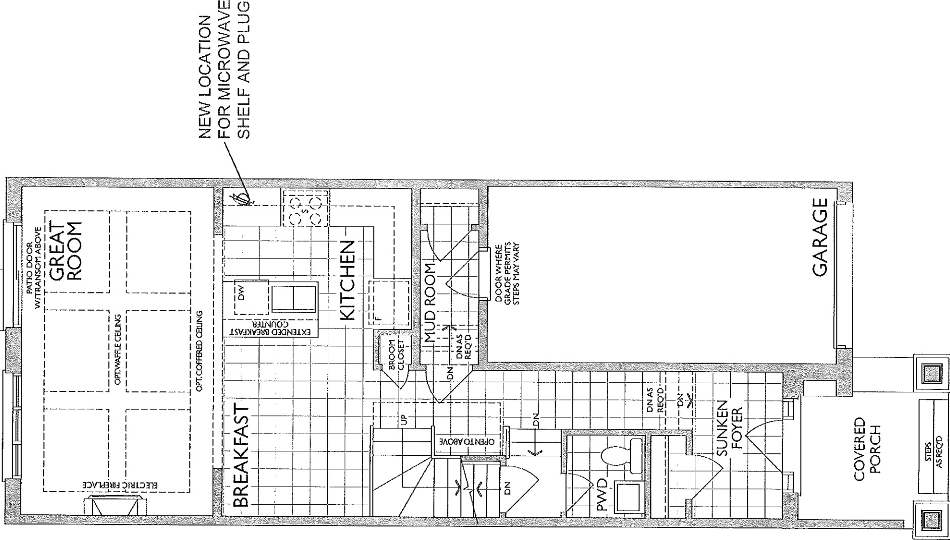
MAIN FLOOR ELEVATION B
