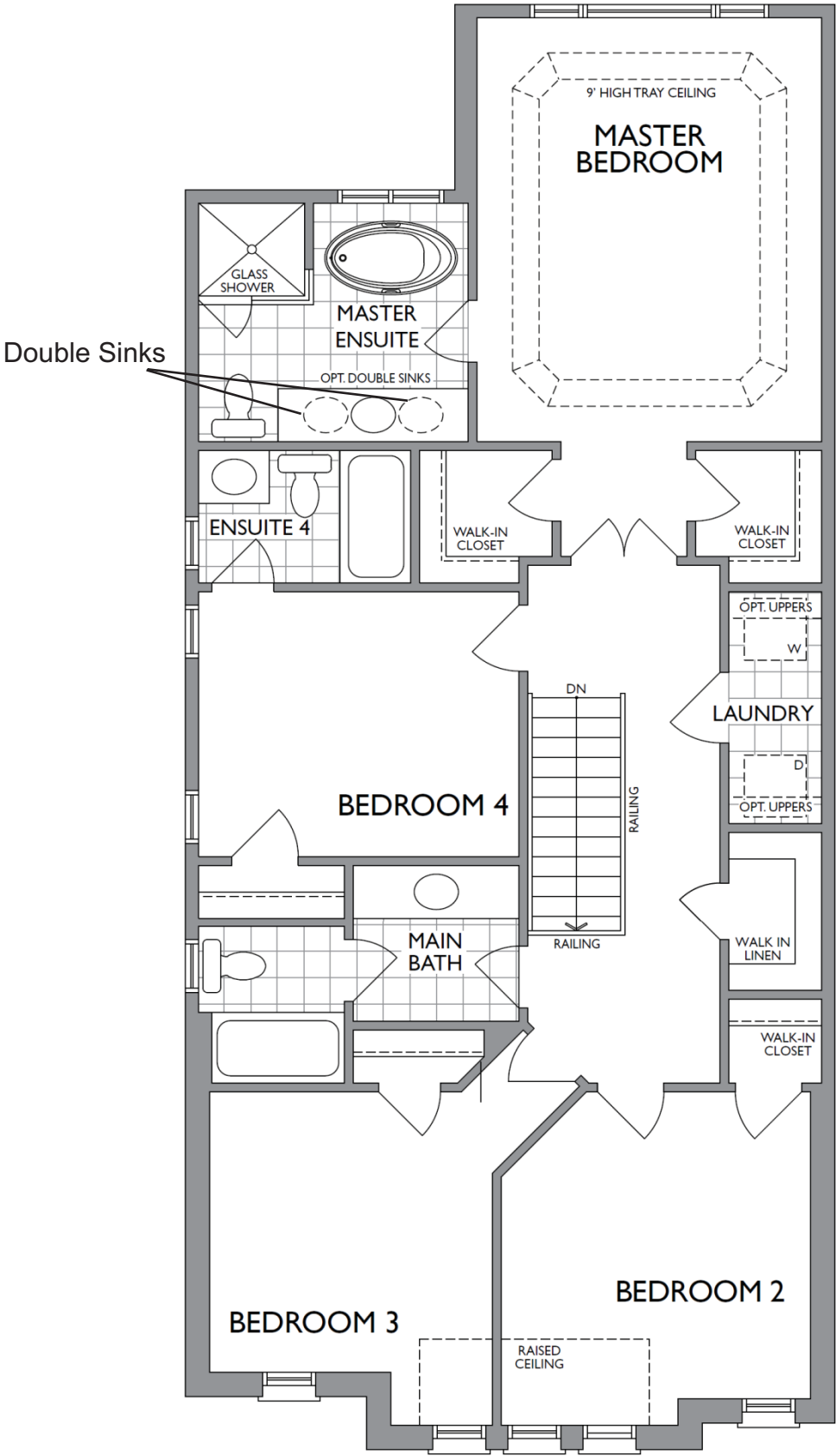
SECOND FLOOR ELEVATION B
