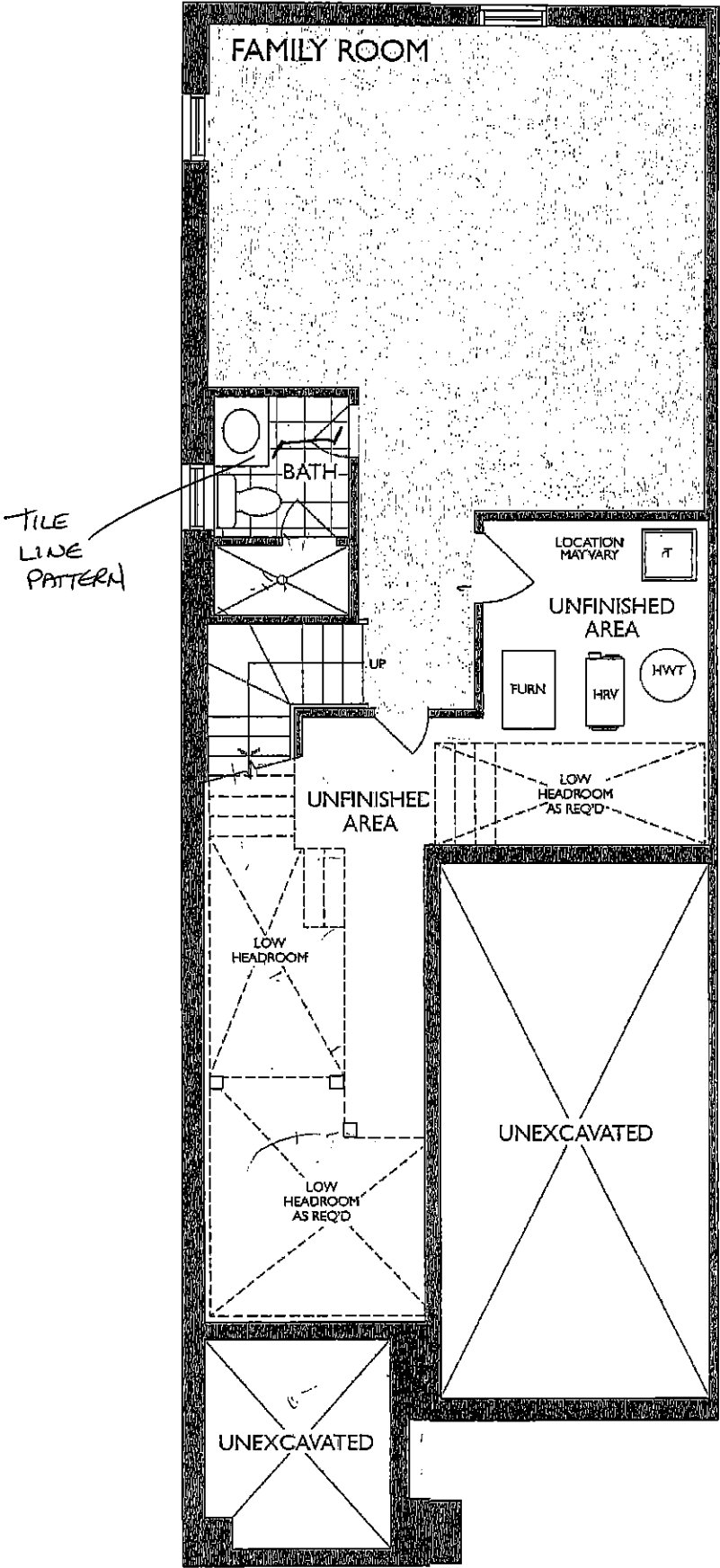
LOWER LEVEL - END ELEVATION A
