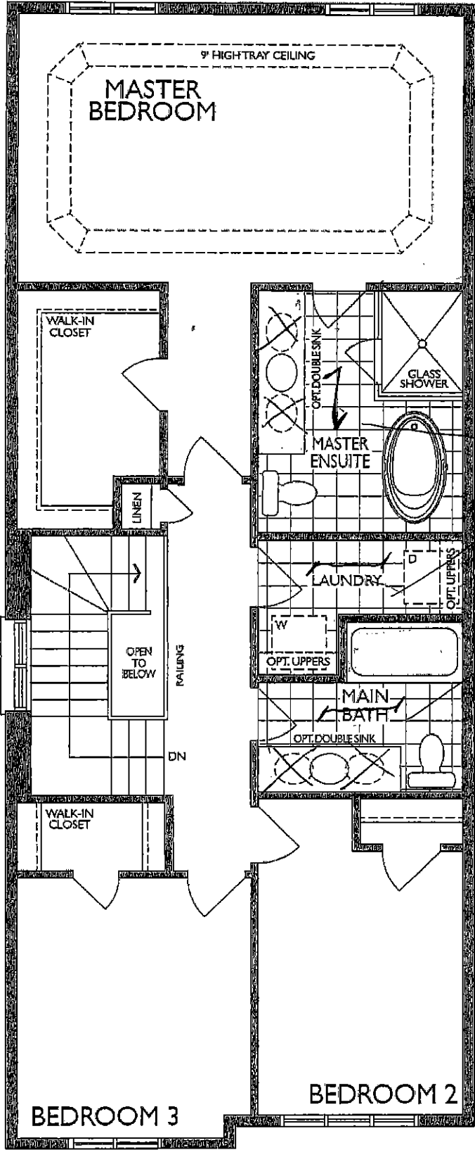
SECOND FLOOR - END ELEVATION A
