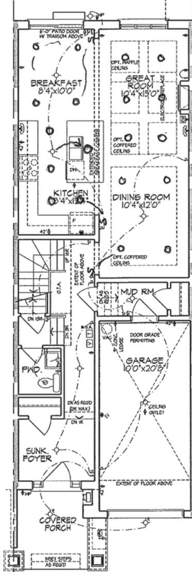
GROUND FLOOR PLAN, ELEV. 'A'
