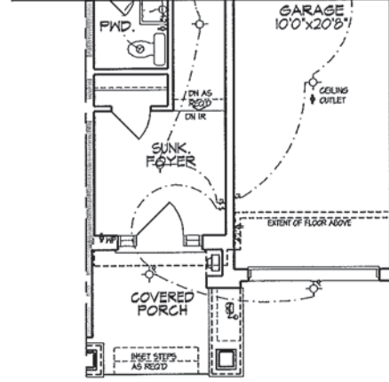
PART. GROUND FLOOR PLAN, ELEV. 'B'
