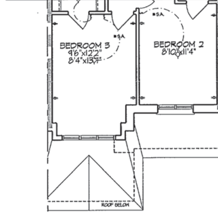
PART. SECOND FLOOR PLAN, ELEV. 'B'
