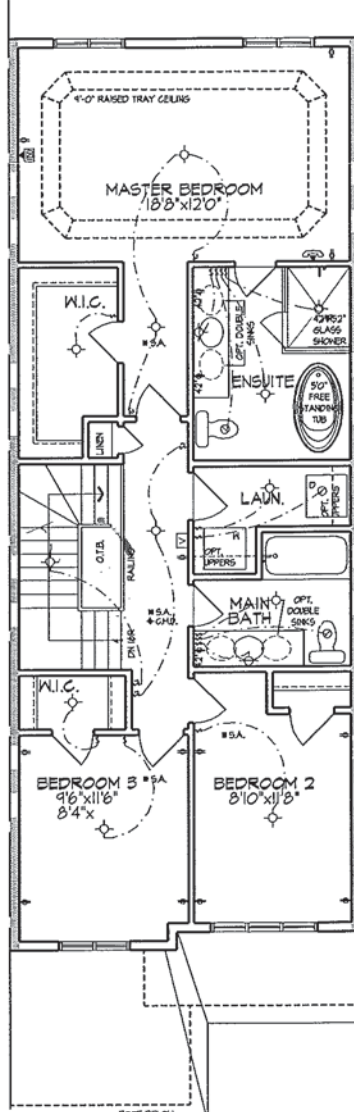
SECOND FLOOR PLAN, ELEV. 'A'
