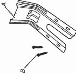
A. Anti-tip bracket B. #12 x 15/16" screws (2)
