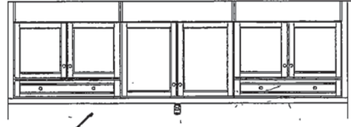
ALT. SHARED BATH E (2ND FLR - ELEV. E)
