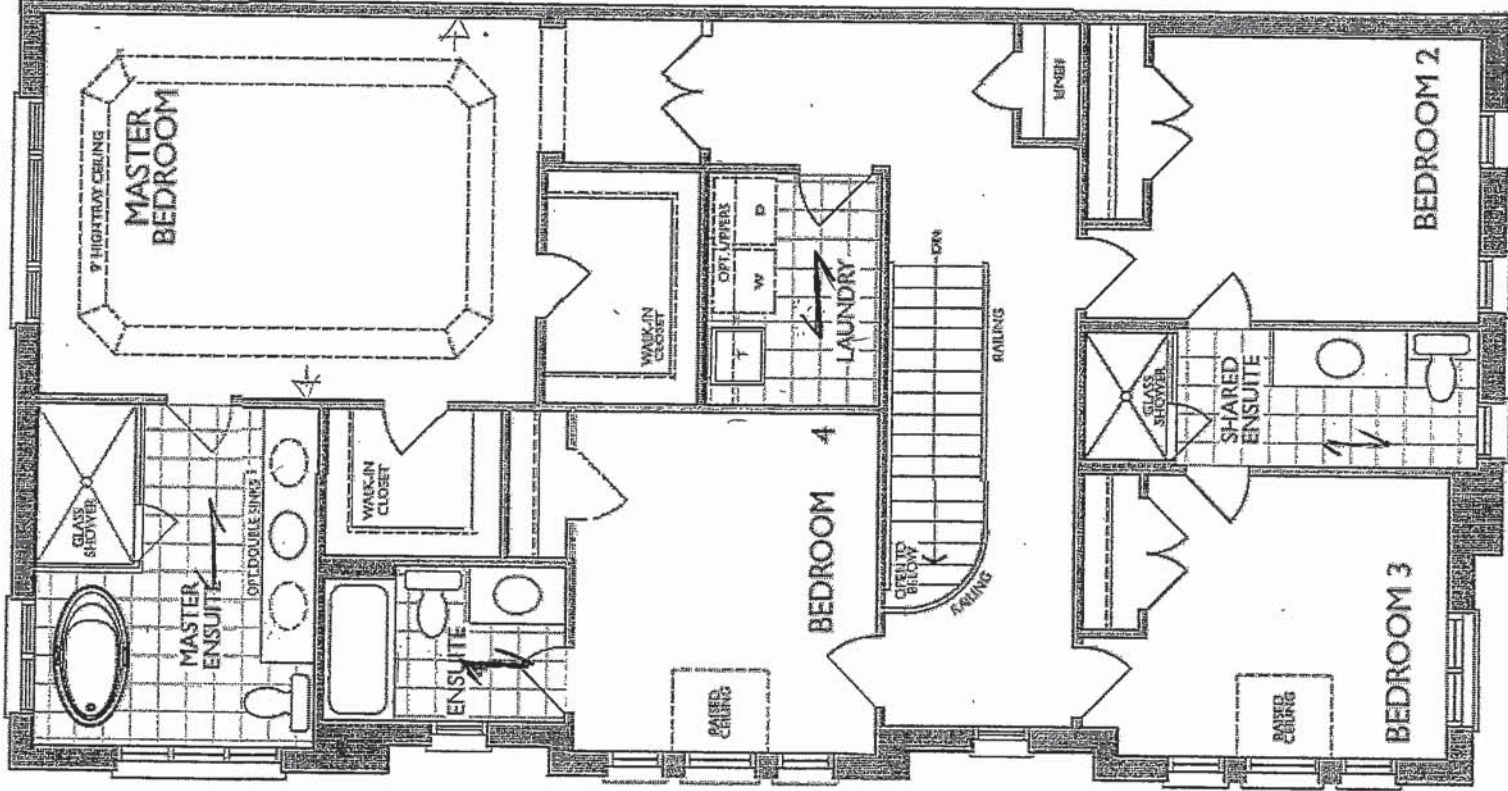
SECOND FLOOR ELEVATION D
