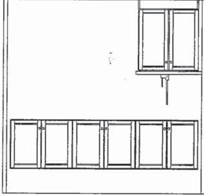
OPT. LAUNDRY UPpers OPT. LAUNDRY BASE (2ND FLR)
