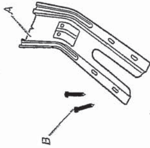
A. Anti-tip bracket B. #12 x 1 5/8" screws (2)
