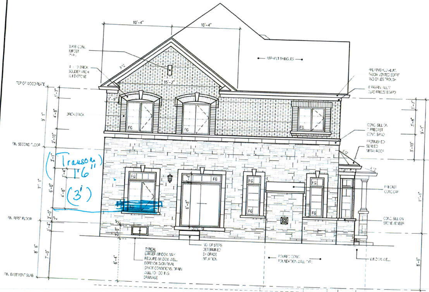
REAR ELEVATION 1
