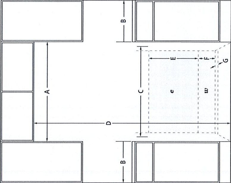
OPENING/CLEARANCE DIMENSIONS
