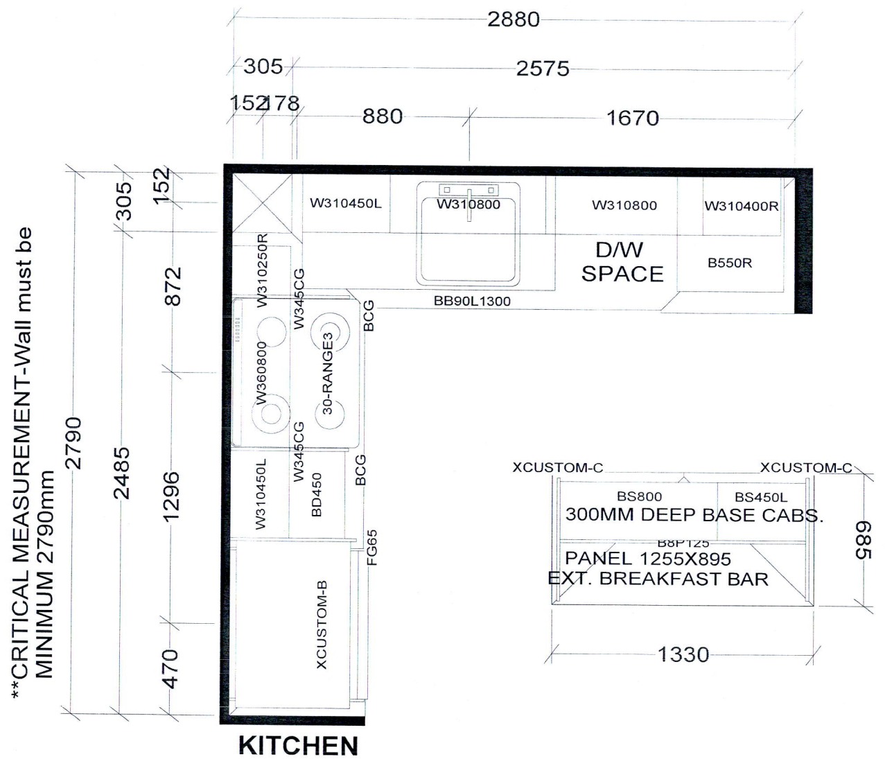
BASE & VANITY CABINETS ON ADJUSTABLE LEGS
