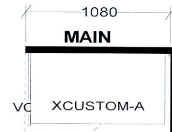
CUSTOM 2 DRAWER VANITY (Drawers modified to clear plumbing) FLOATING TOEKICK
