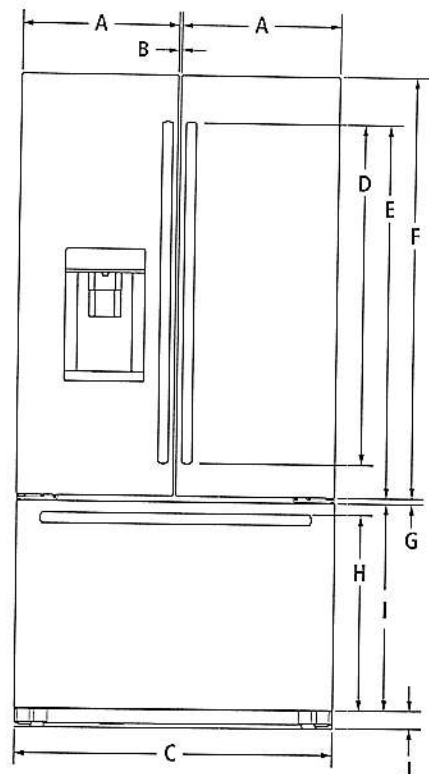
FRONT VIEW
