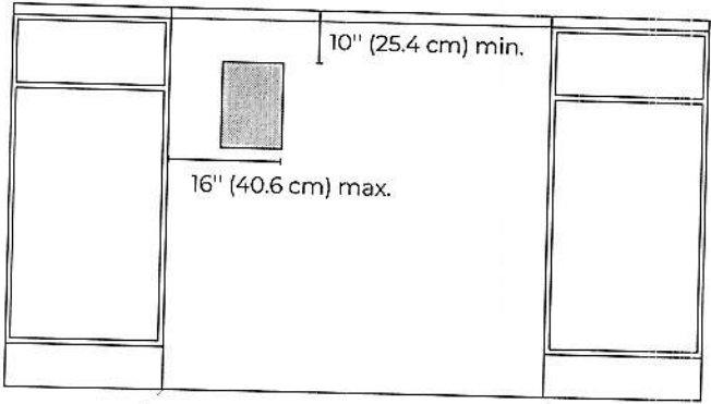
RECOMMENDED ELECTRICAL OUTLET ZONE
