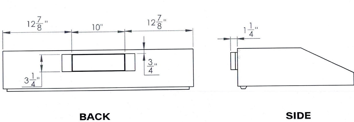
Horizontal Adapter
