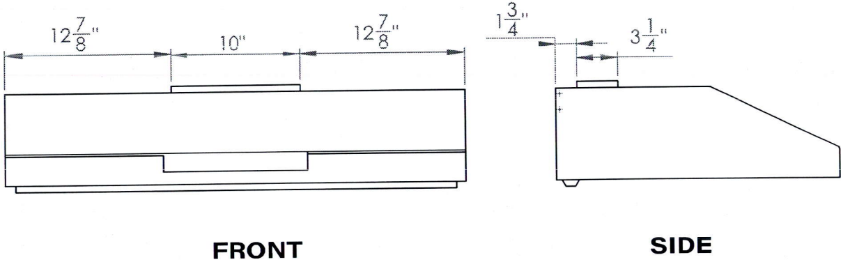
Vertical adapter
