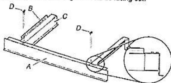
A. Bottom vent B. Spacer bar flange C. Spacer bars D. \frac{3}{8} " (9.5 mm) hex-head washer screws
