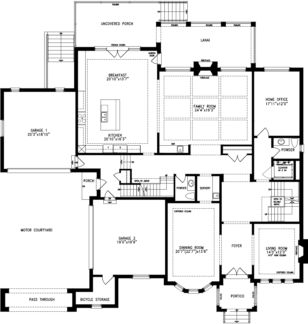
MAIN LEVEL
