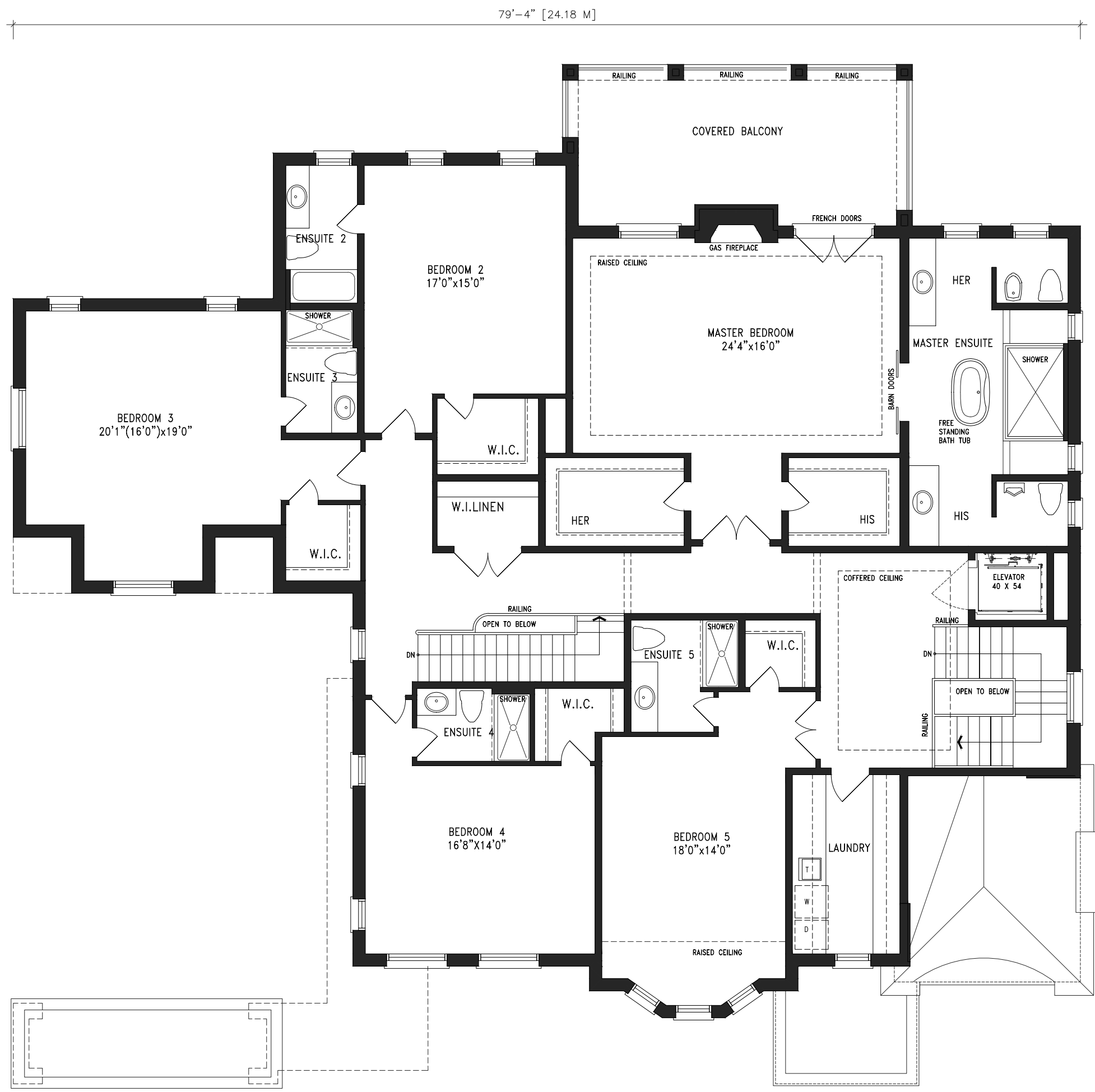
SECOND FLOOR PLAN 1
