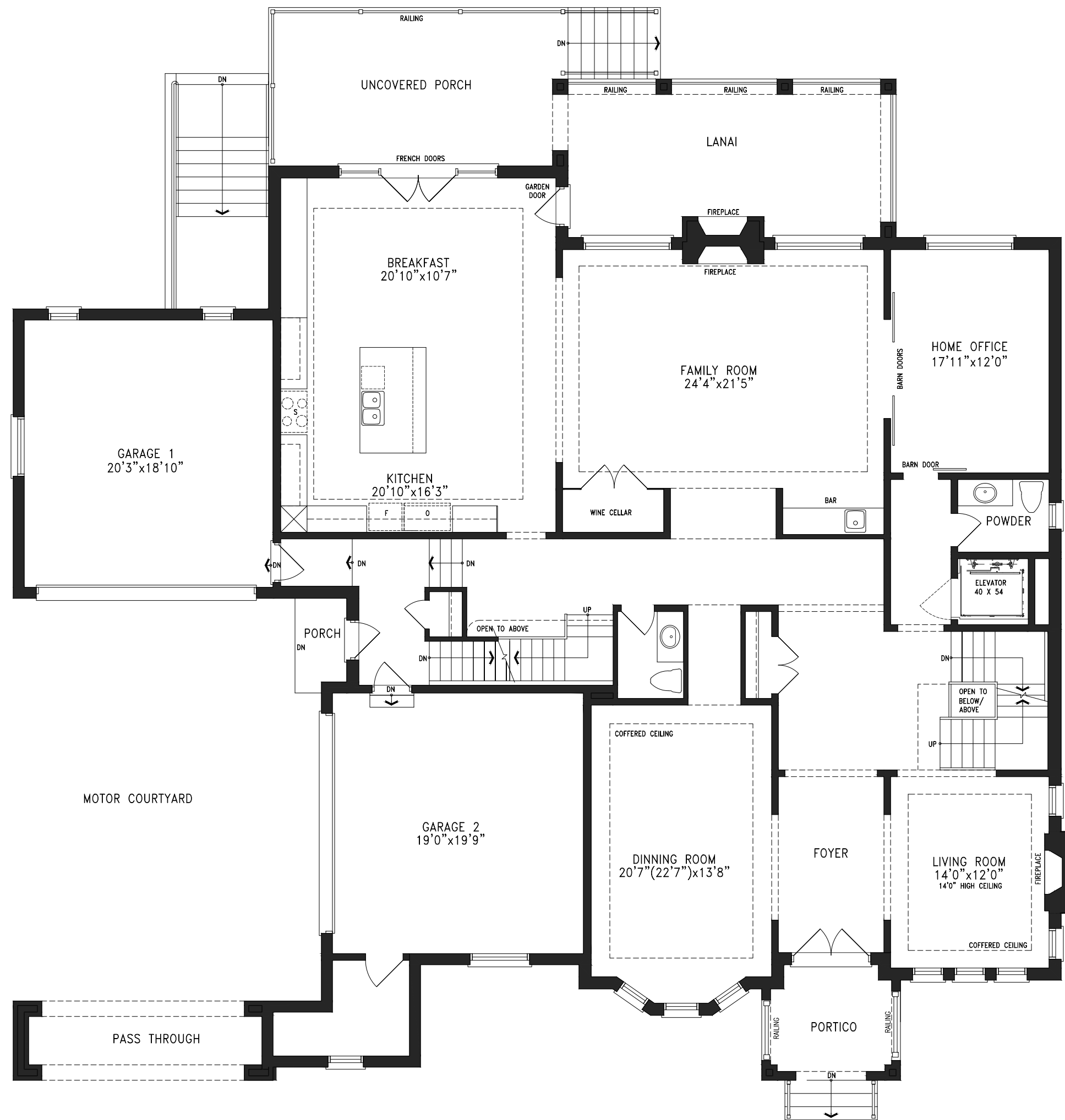
FIRST FLOOR PLAN 1
