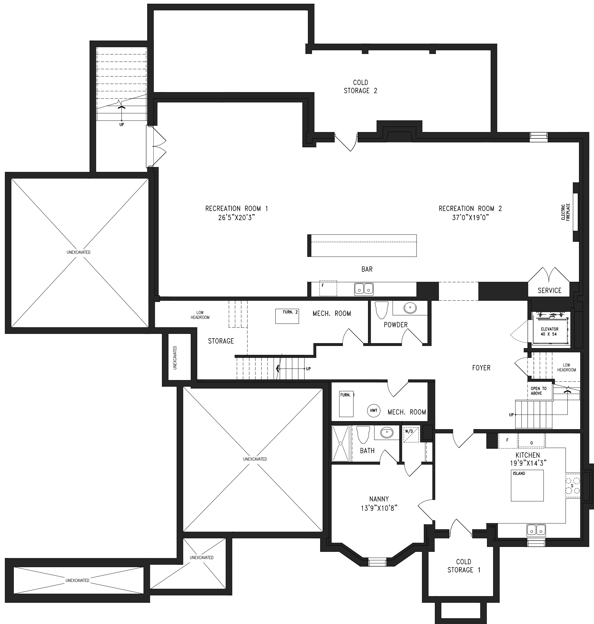
BASEMENT PLAN 1 FINISHED AREA= 2,355 SQ.FT.
