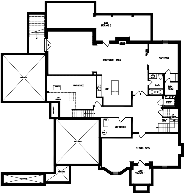
LOWER LEVEL
