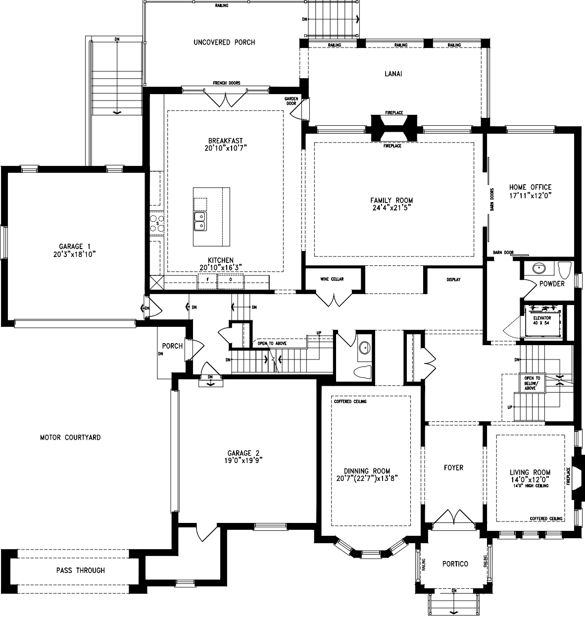
MAIN LEVEL
