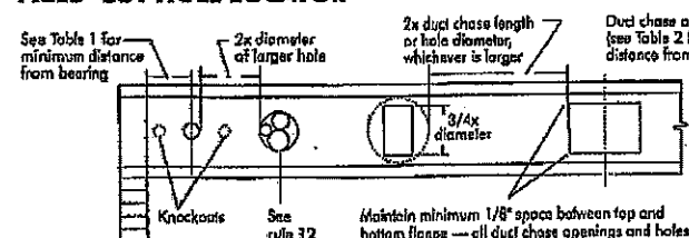
FIGURE 7 FIELD-CUT HOLE LOCATOR
