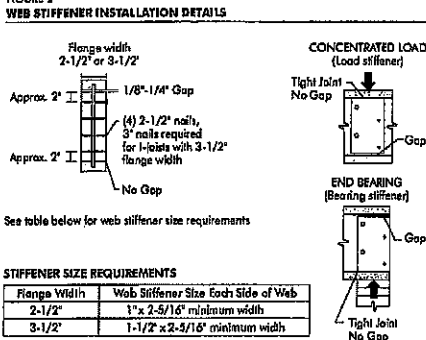
FIGURE 2 WEB STIFFENER INSTALLATION DETAILS
