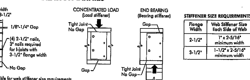
FIGURE 2 WEB STIFFENER INSTALLATION DETAILS
