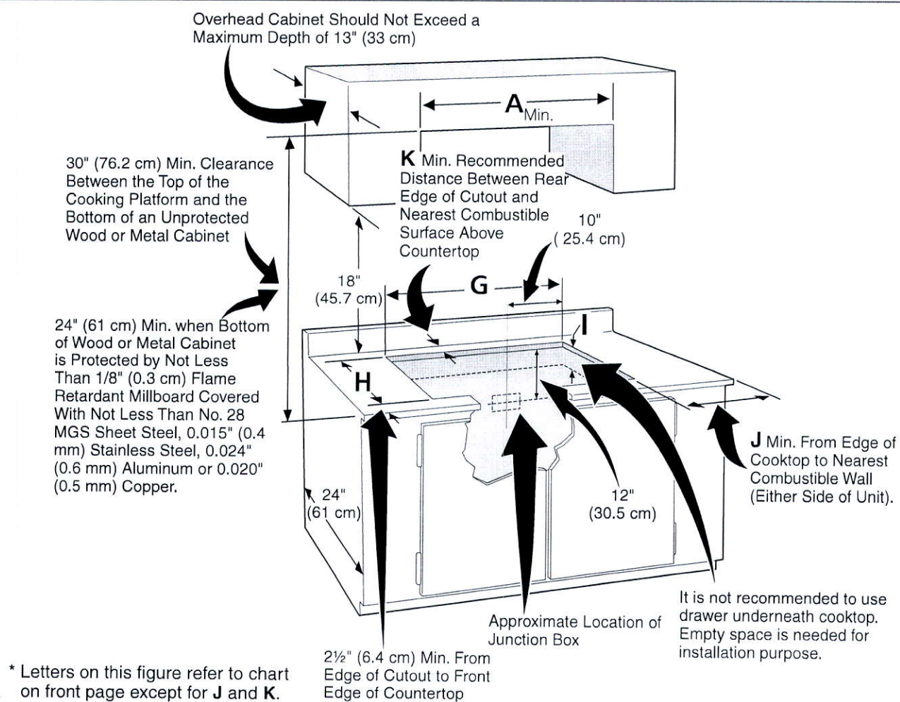
Figure 2 – COUNTERTOP CUTOUT OPENING
