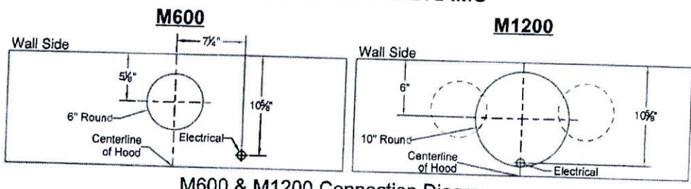
M600 & M1200 Connection Diagrams
