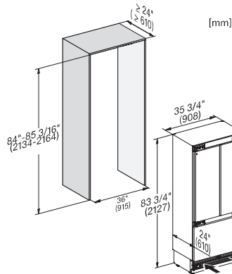
KF2982Vi, KF2981Vi, installation, MasterCool, installation drawings
