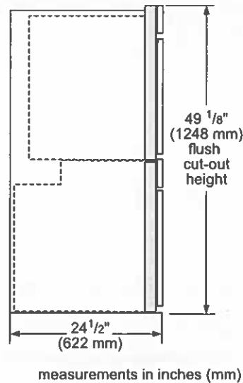
Side View-Combination Oven with Microwave or Speed Oven
