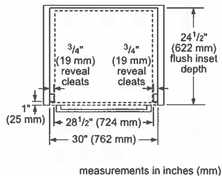
Combination Oven with Microwave or Speed Oven, flush mount installation Top View Bottom Hinge Door
