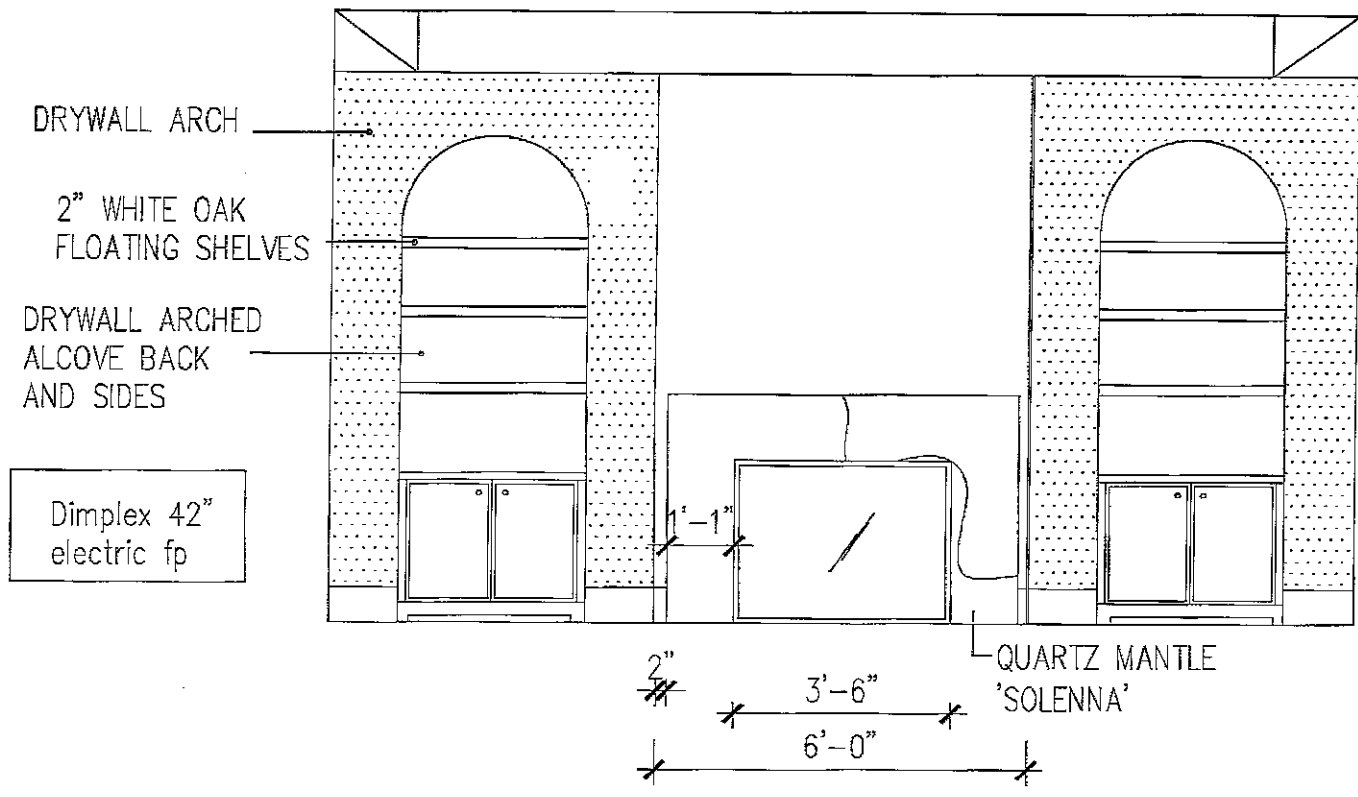
TM-16-4 GREAT ROOM - FIREPLACE PART PLAN AND ELEVATION
