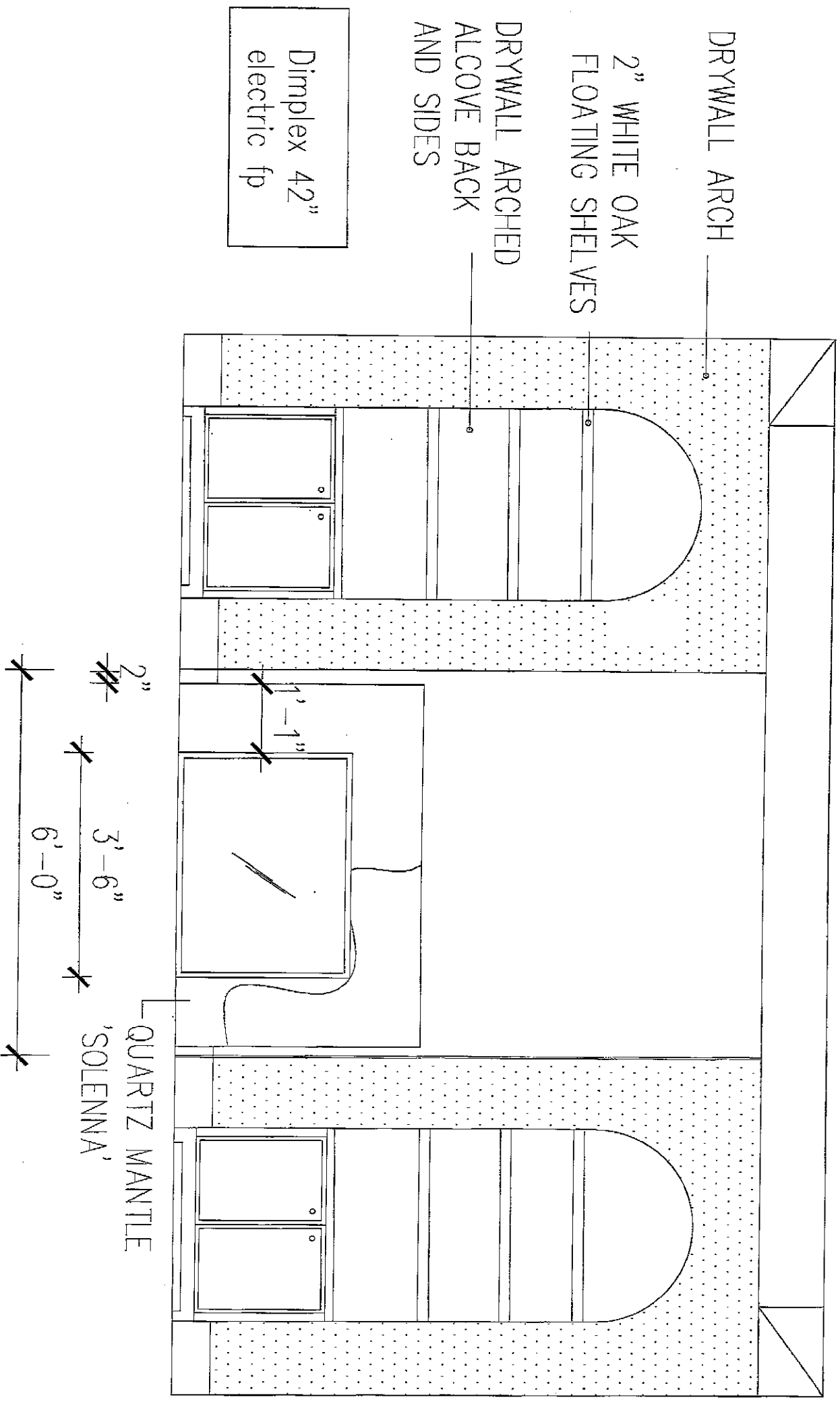
TM-16-4 GREAT ROOM - FIREPLACE PLAN AND ELEVATION
