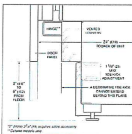
Toe Kick (side view).
