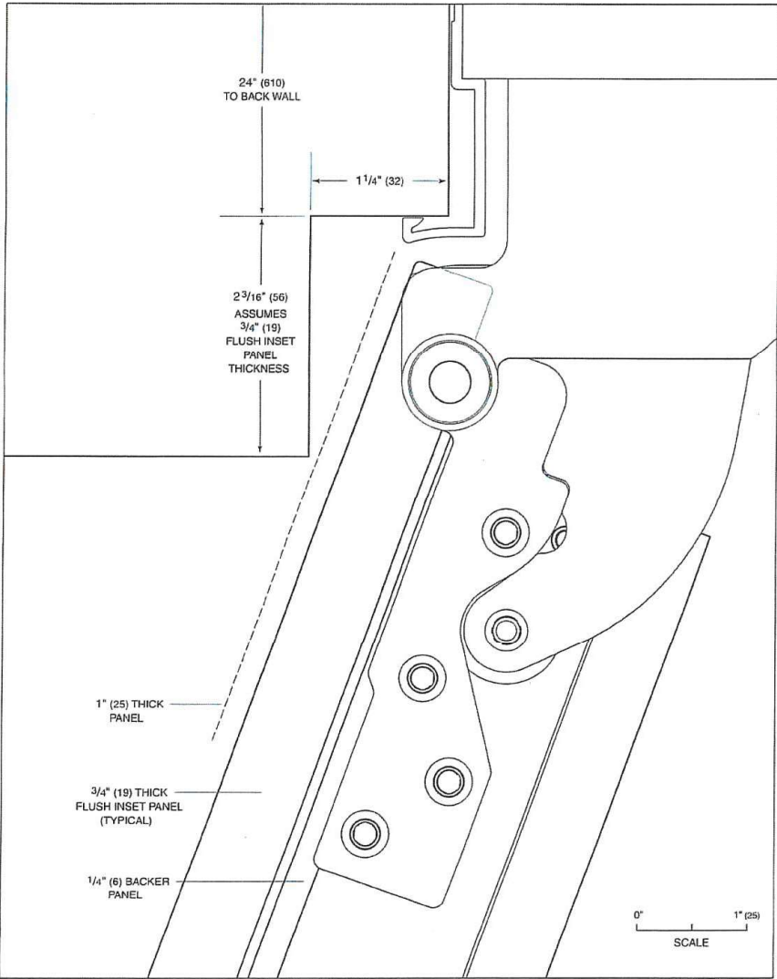
Flush inset application—110° door opening (top view).
