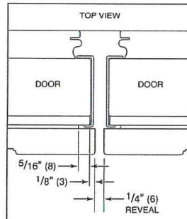
Doors (handle) Sides
