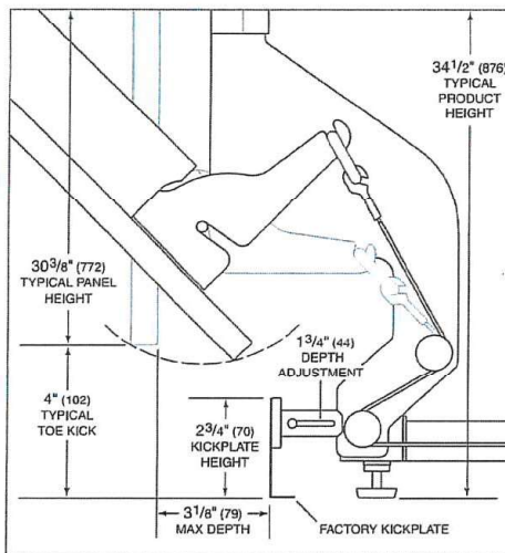
Toe kick area (side view)
