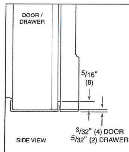
Door/Drawer Bottom
