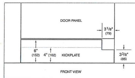
Kickplate notch
