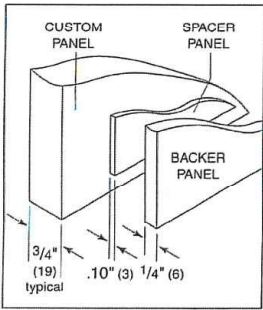
Panel assembly (rear view).
