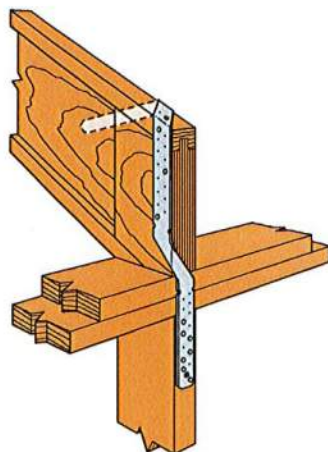
MTS30 Installation with I-Joist Rafter
