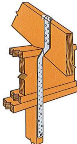
Typical MTS30 Installation
