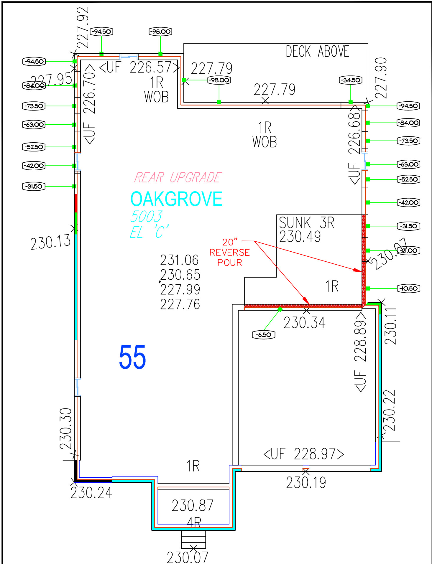
PLAN
