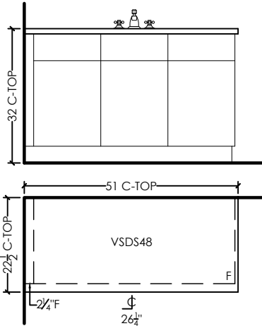
ENSUITE 3 5 BDRM (ELEV C) DESIGN: STAIN: HDWE: CTOP: ¾" SLAB BY OTHERS DRAWER TRACKS: STANDARD CABINET HEIGHT: 32" HIGH
