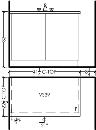
ENSUITE 4 (5 BDRM ELEV B) DESIGN: STAIN: HDWE: CTOP: ¾" SLAB BY OTHERS CABINET HEIGHT: 32" HIGH
