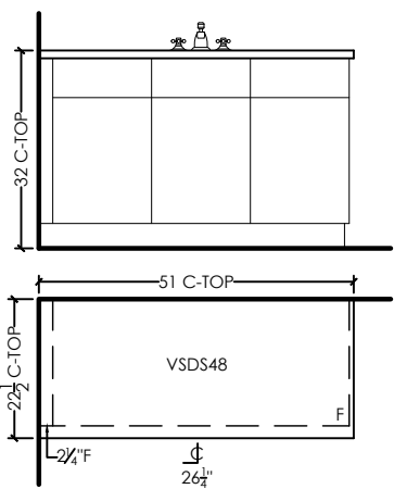
PART. 2ND FLR ENS 3 W/LOFT DESIGN: STAIN: HDWE: CTOP: ¾" SLAB BY OTHERS DRAWER TRACKS: STANDARD CABINET HEIGHT: 32" HIGH
