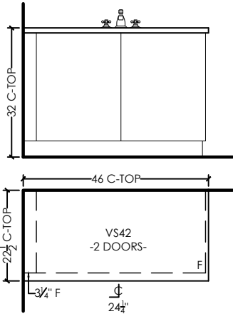
PART 2ND FLR ENS 3 (ELEV B) DESIGN: STAIN: HDWE: CTOP: ¾" SLAB BY OTHERS CABINET HEIGHT: 32" HIGH
