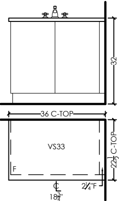
ENSUITE 4 5 BDRM (ELEV C) DESIGN: STAIN: HDWE: CTOP: ¾" SLAB BY OTHERS CABINET HEIGHT: 32" HIGH
