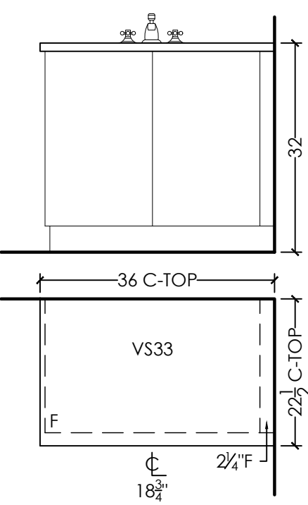
OPT. BASEMENT BATH DESIGN: STAIN: HDWE: CTOP: 3/4" SLAB BY OTHERS CABINET HEIGHT: 32" HIGH
