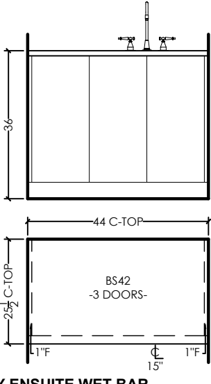
OPT. PRIMARY ENSUITE WET BAR DESIGN: STAIN: HDWE: CTOP: 3/4" SLAB BY OTHERS CABINET HEIGHT: 36" HIGH
