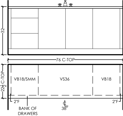
ENSUITE 4 DESIGN: STAIN: HDWE: CTOP: 3/4" SLAB BY OTHERS CABINET HEIGHT: 32" HIGH
