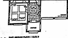
PART GROUND FLOOR | ELEV. B
