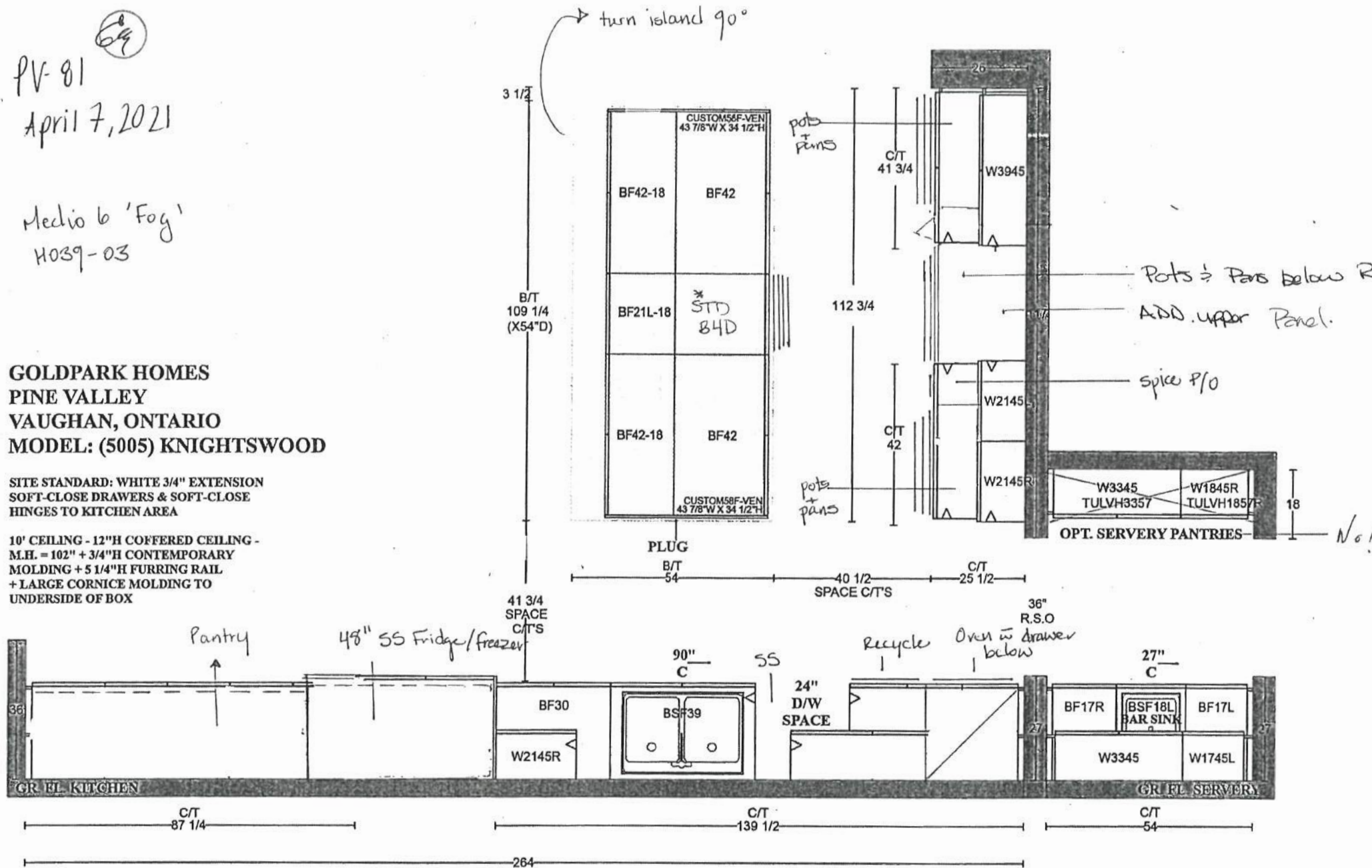
PLAN VIEW
