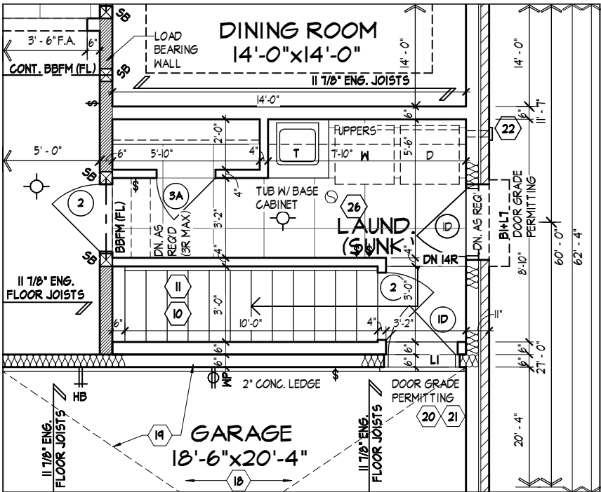
PART. GROUND FLOOR PLAN, ELEV. 'A' W/ OPT. SERVICE STAIR (8' BASEMENT COND.)-LOT 18
