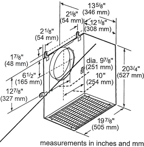
VTR1030W-1000 CFM
