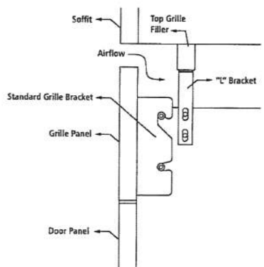
SIDE VIEW – CUSTOM PANEL
