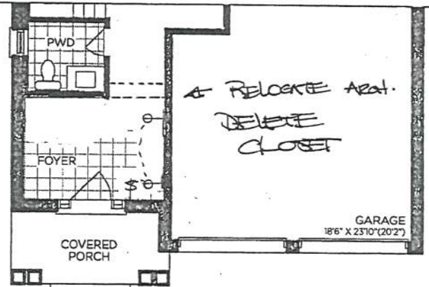
PART. GROUND FLOOR | ELEV. B
