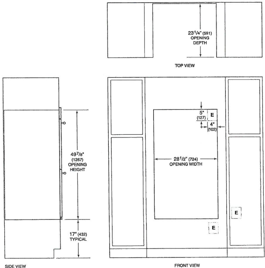
SIDE VIEW
