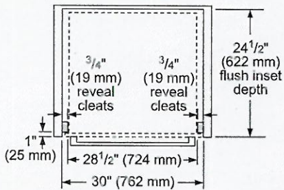
Combination Oven with Microwave or Speed Oven, flush mount installation Top View Bottom Hinge Door
