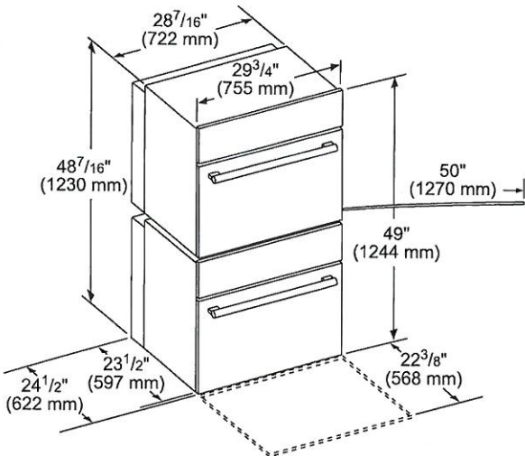
Combination Oven with Microwave or Speed Oven
