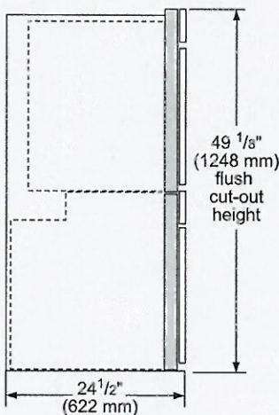
Side View-Combination Oven with Microwave or Speed Oven
