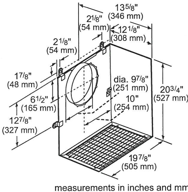
VTR1330W-1300 CFM
