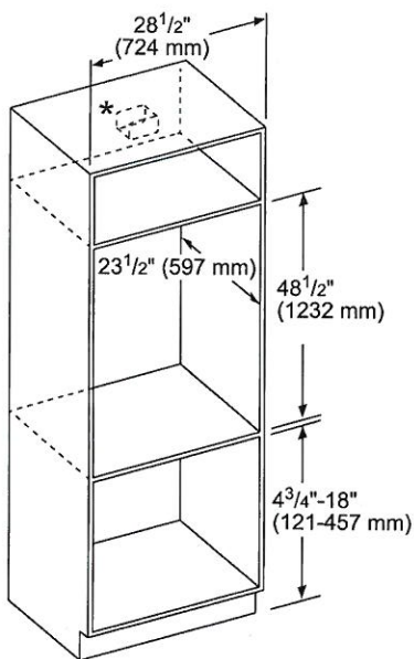
Combination Oven with Microwave or Speed Oven
