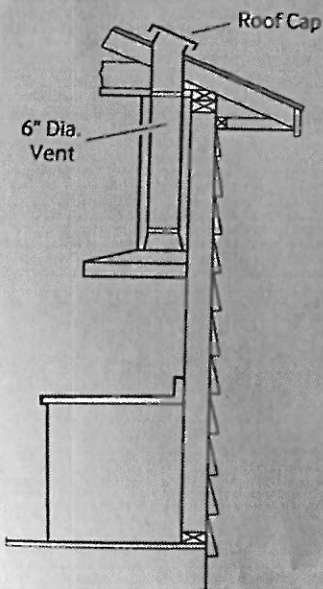
Roof Venting
