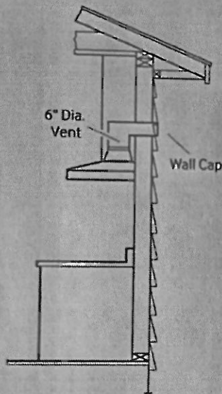
Wall Venting
