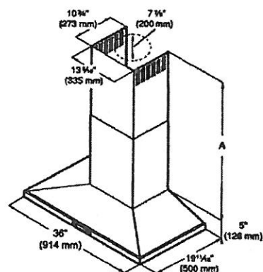
A Ducted operation: Min. / Max. 24 9/16" (624 mm) / 36 7/8" (935 mm) Recirculation mode: Min. / Max. 28 1/4" (716 mm) / 42 9/16" (1081 mm) measurements in inches (mm)
