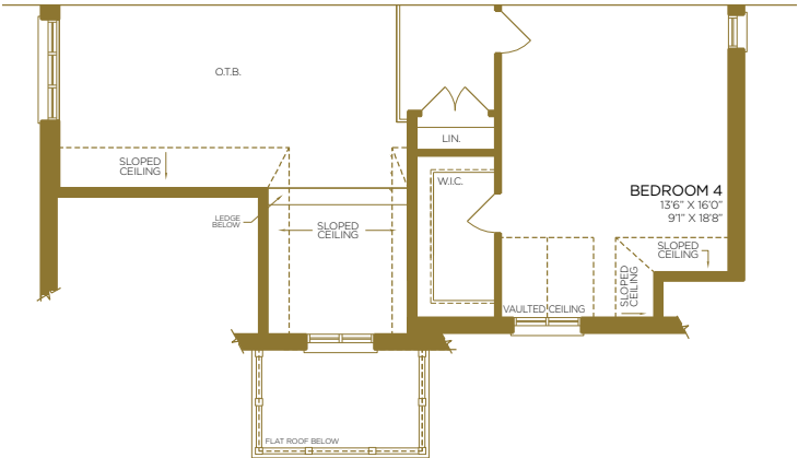
PART. SECOND FLOOR | ELEV. B
